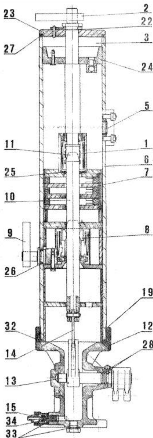
Slika 1 – Presjek pola prekidača tip HG4/7C, HG4/7F, HG4a/8C, HG4a/8F HG6a/8C, HG6a/8F, HG6as/8C, HG6as/8F
